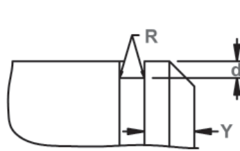
Exploded Groove Profile & Edge Margin (Y) Maximum bottom radii (R), .005 for ring sizes -39 thru -98; -.010 for ring sizes -106 thru -200
