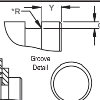
Maximum Corner Radius & Chamfer
