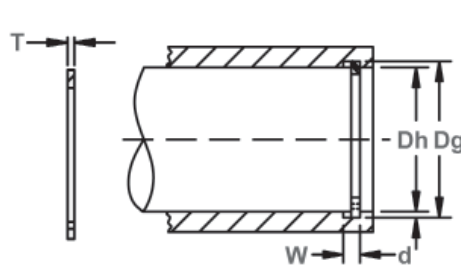
Housing Diameter & Groove Dimensions
