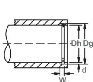
Allowable Diameter & Groove Dimensions
