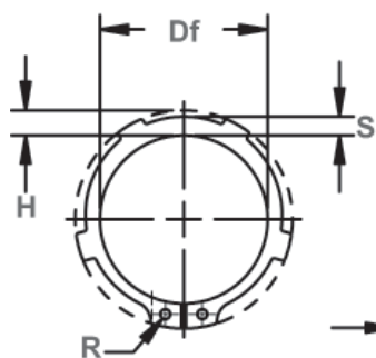
Free Diameter & Ring Measurements With Section B-B
