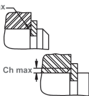
Maximum Corner Radius & Chamfer
