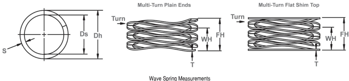
Wave Spring Measurements
