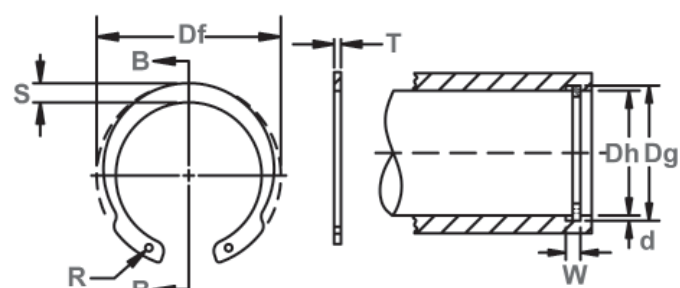
Free Diameter & Ring Measurements With Section B-B
