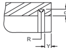
Exploded Groove Profile & Edge Margin (Y) Maximum bottom radii (R), .005 for ring sizes -25 thru -100; .010 for ring sizes -102 and over
