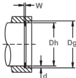
Housing Diameter & Groove Dimensions
