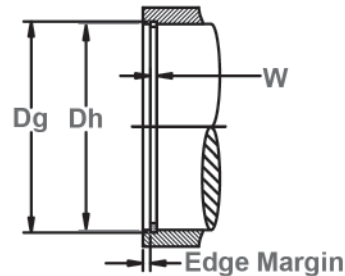
Housing Diameter & Groove Dimensions
