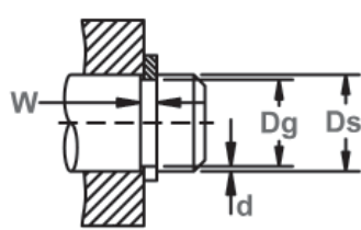
Shaft Diameter & Groove Dimensions
