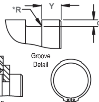
Alternate Design Manufacturer's Option
