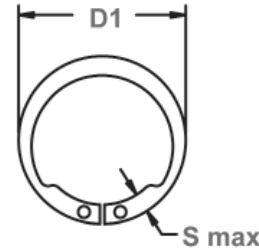
Measuring Free Diameter (Df) SHI Series Df = D1 - 2(S max)
