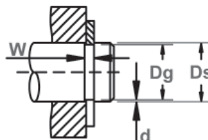
Optional Use in Groove (Larger Sizes)
