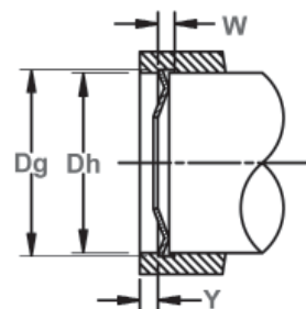
Installation View With Groove
