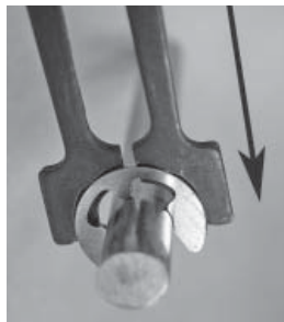
Radial Installation.
