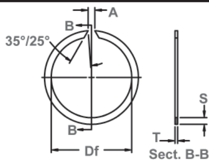
Free Diameter & Ring Measure
