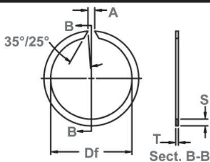
Free Diameter & Ring Measure
