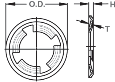
RTX Prong Configuration
