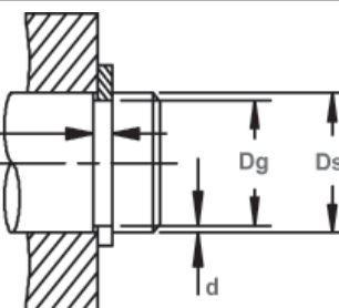
Shaft Diameter & Groove Dimensions
