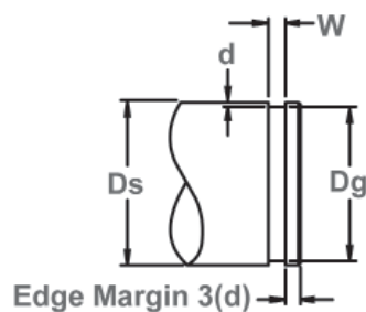
Shaft Diameter & Groove Dimensions
